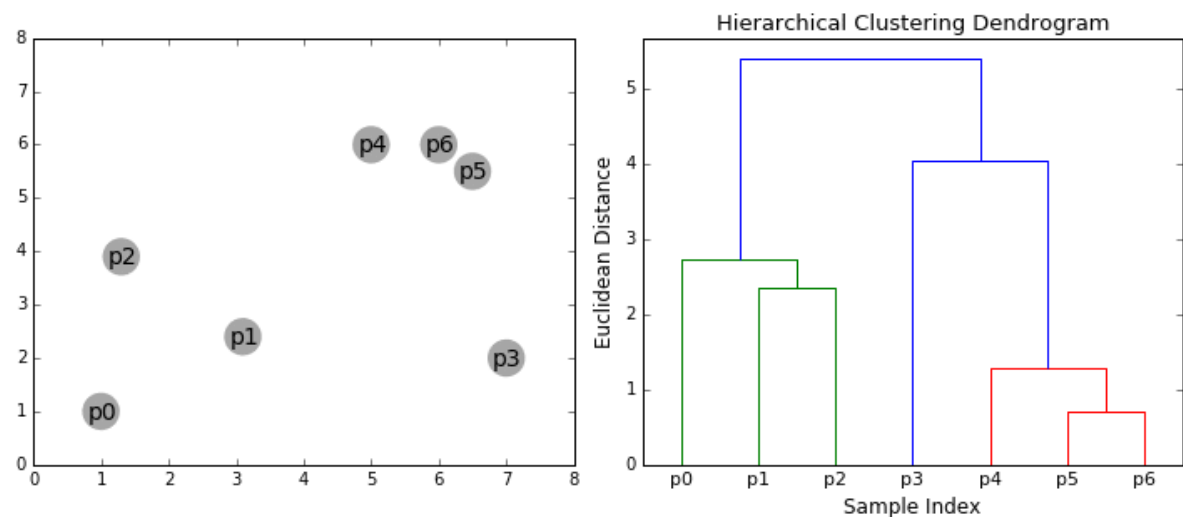
Agglomerative Hierarchical Clustering
