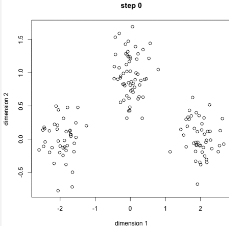
K-Means Clustering
