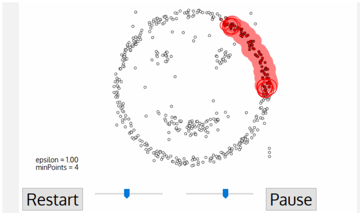
DBSCAN Smiley Face Clustering
